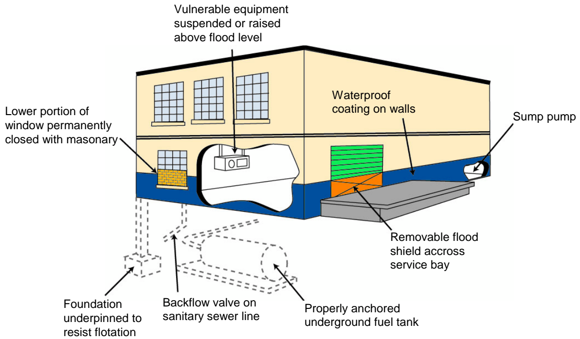
Figure 1 – Dry flood proofing
