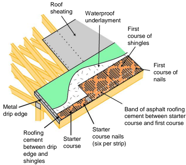
Figure 4 – Secured composition shingles
