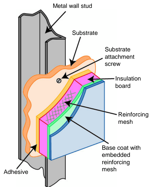
Figure 6 – EIFS Wall
