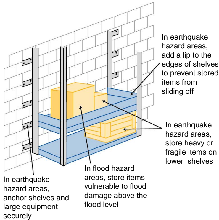
Figure 8 – Secured equipment
