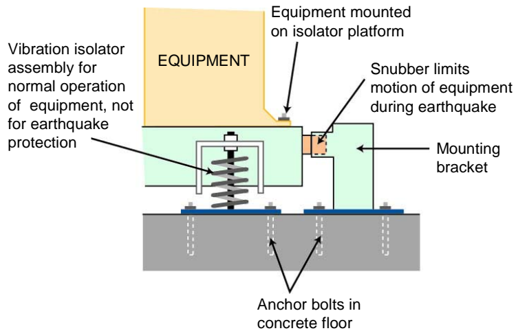
Figure 9 – Anchored equipment
