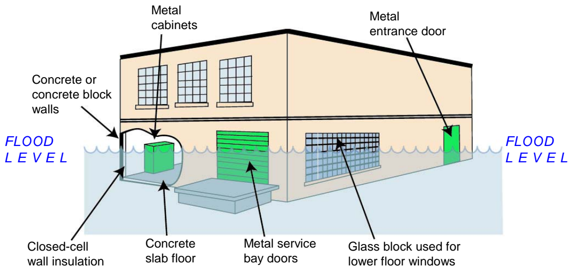
Figure 2 – Flood-resistant materials
